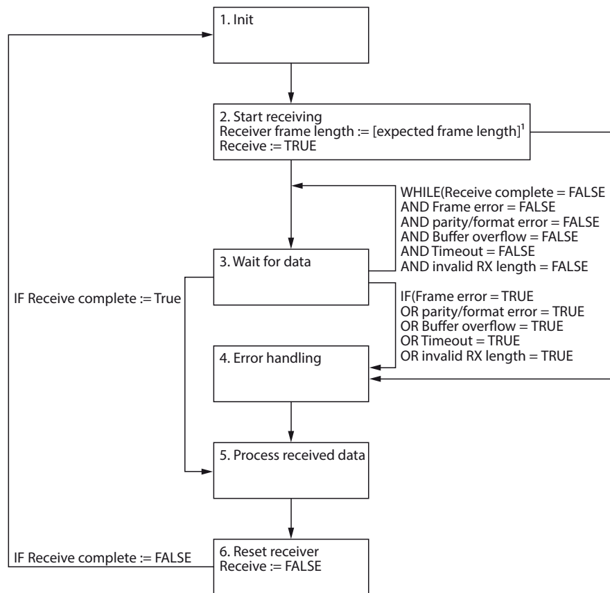
Fig. 73: Receive sequence
