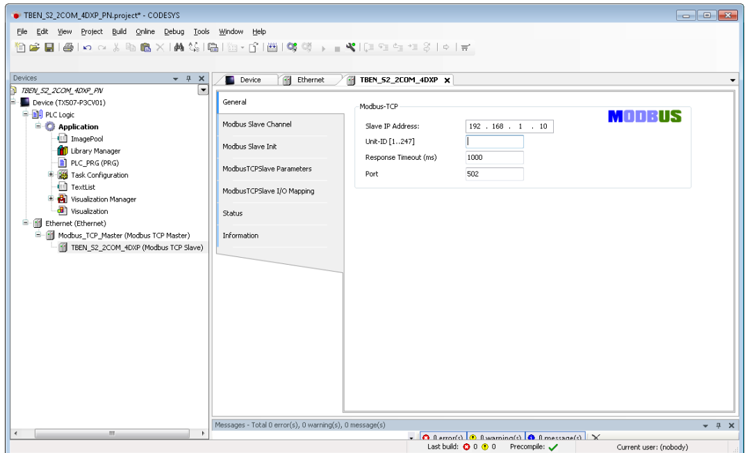
Fig. 61: Modbus TCP-Slave – entering the IP address
