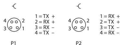
Fig. 13: Pin assignment Ethernet connectors
