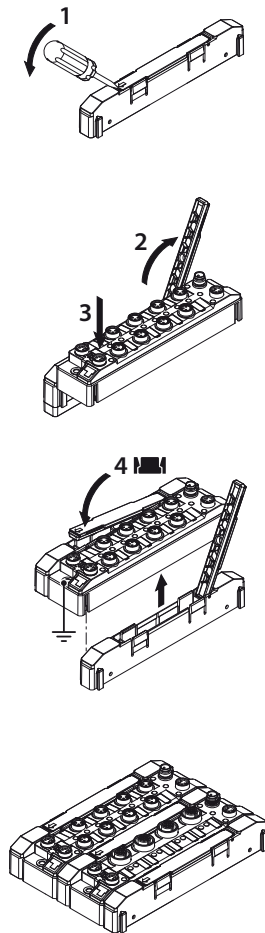
Fig. 2: Build module groups four mounting the devices onto a mounting plate
