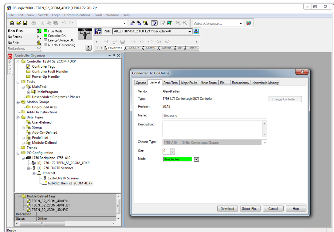
Fig. 47: Clicking "Download"
