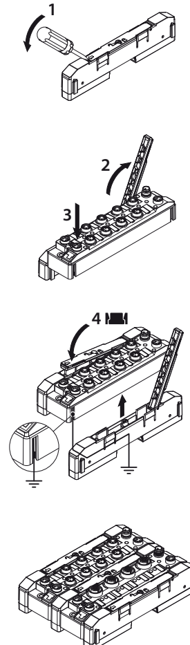
Fig. 3: Build module groups four mounting the devices onto a DIN rail (TS35)
